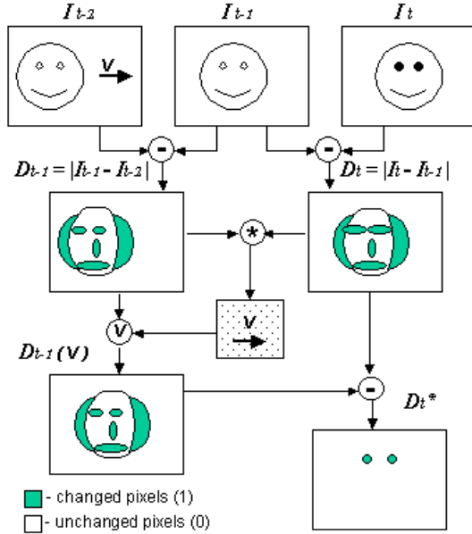
Fig. 3. A flowchart for detection eye blinks using with second order change detection.
